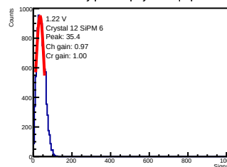
ADC-only | 1.22 V | crystal 12 | sipm 6
