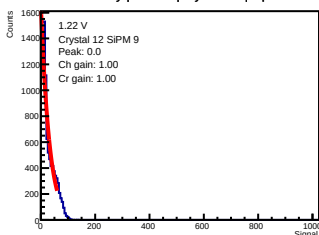
ADC-only | 1.22 V | crystal 12 | sipm 9
