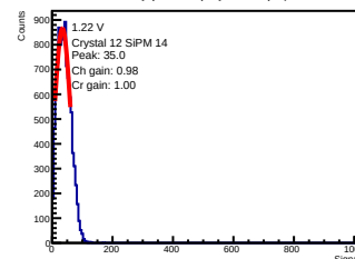
ADC-only | 1.22 V | crystal 12 | sipm 14
