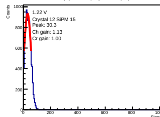
ADC-only | 1.22 V | crystal 12 | sipm 15
