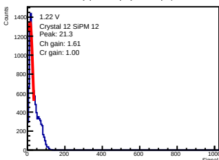
ADC-only | 1.22 V | crystal 12 | sipm 12
