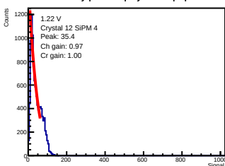
ADC-only | 1.22 V | crystal 12 | sipm 4
