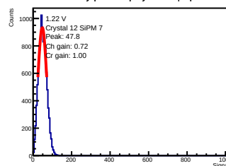
ADC-only | 1.22 V | crystal 12 | sipm 7
