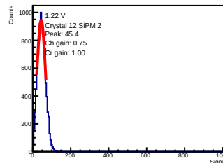
ADC-only | 1.22 V | crystal 12 | sipm 2
