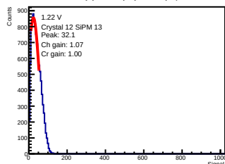
ADC-only | 1.22 V | crystal 12 | sipm 13
