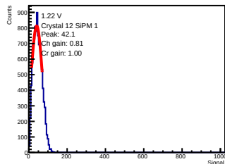
ADC-only | 1.22 V | crystal 12 | sipm 1
