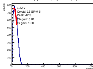
ADC-only | 1.22 V | crystal 12 | sipm 5
