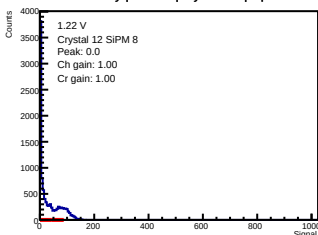
ADC-only | 1.22 V | crystal 12 | sipm 8
