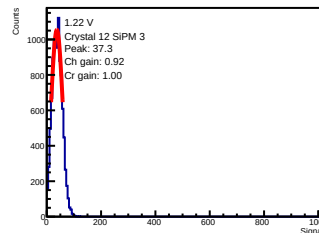
ADC-only | 1.22 V | crystal 12 | sipm 3
