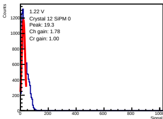
ADC-only | 1.22 V | crystal 12 | sipm 0
