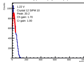
ADC-only | 1.22 V | crystal 12 | sipm 10
